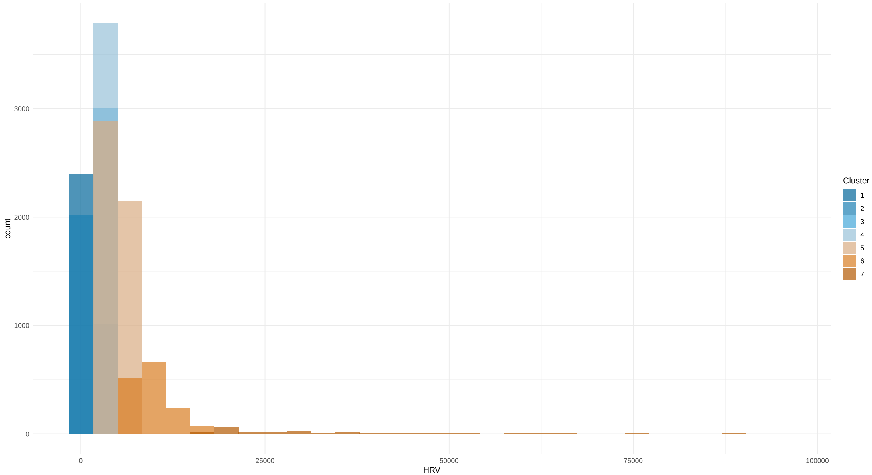
HRV clustered into automatic groups
